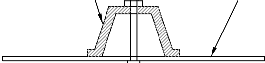
U CHANNEL CONSTRUCTION
