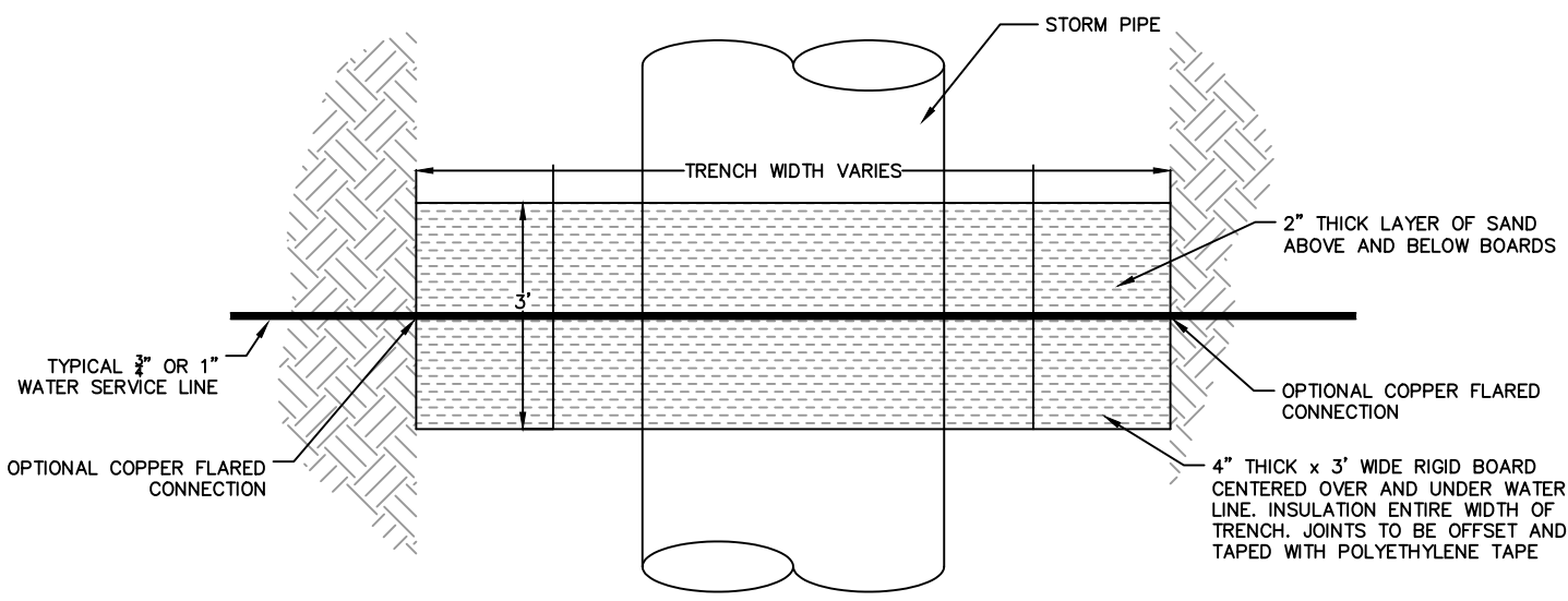
PLAN DETAIL
