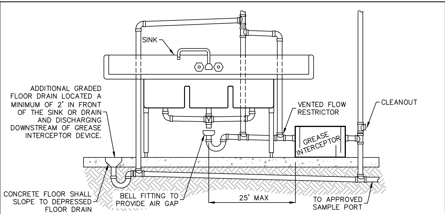
INTERIOR ABOVE GRADE GREASE INTERCEPTOR
