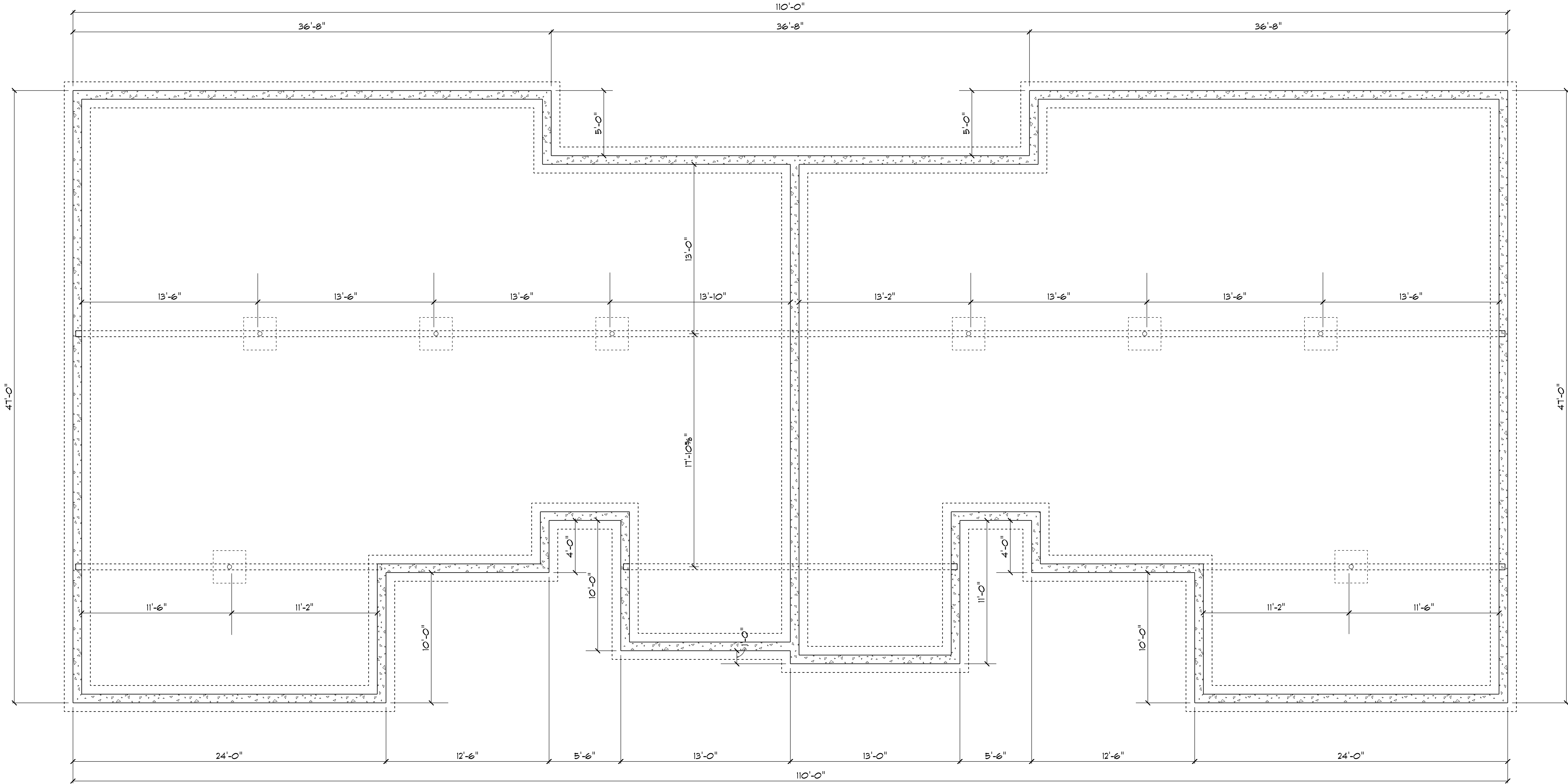
FOUNDATION SCALE: 1/4" = 1'-0"
