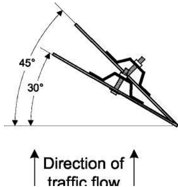
Figure 8 - Angle of signs to oncoming traffic
